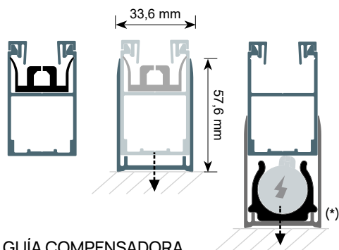
GUÍA COMPENSADORA COULISSE COMPENSATOIRE Counter-balancing fitting for the guide rail
